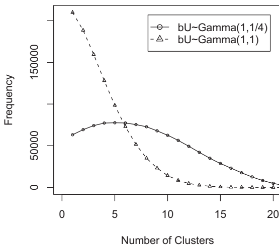
(b) Prior number of clusters integrating over b_U
