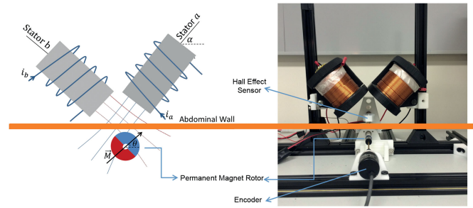
Fig. 5. Electromagnet coils replacing PMs in the external actuation unit for higher level control in LEMA [86].
