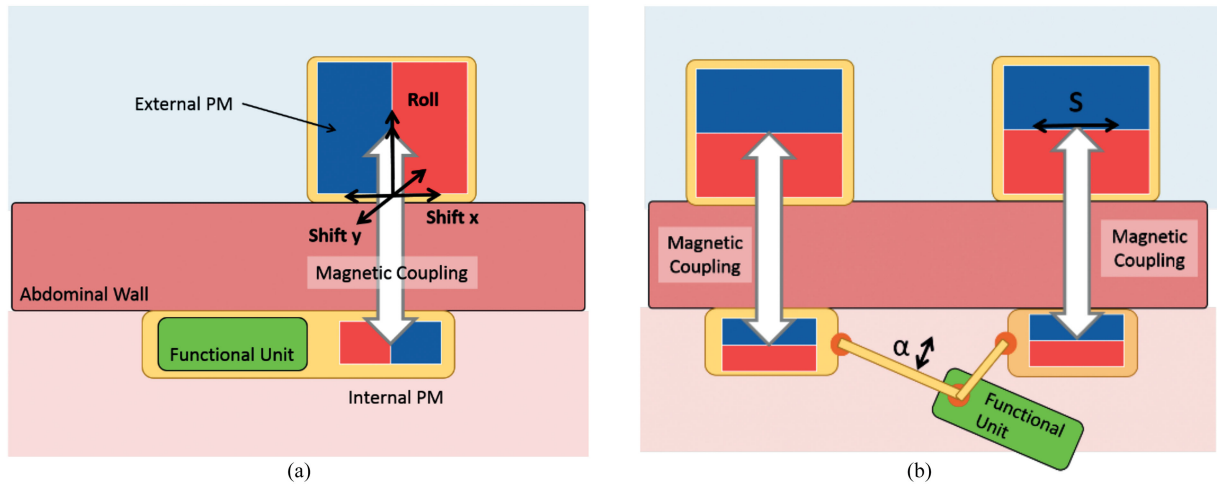
Fig. 2. Illustration of MAGS. (a) MAGS principle of operation. (b) MAGS magnetically actuated by magnetic translation.
