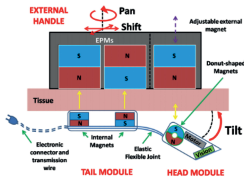
Fig. 7. LMA laparoscopic camera with fine tuning capabilities by Simi et al. [90].
