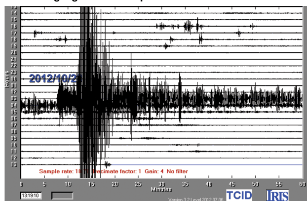
Fig. 3. Snapshot of the seismic data recorded on station TCID in Eagle, ID, on Oct. 28, 2012, when an earthquake struck off the west coast of Canada at 03:04:08 UTC.
