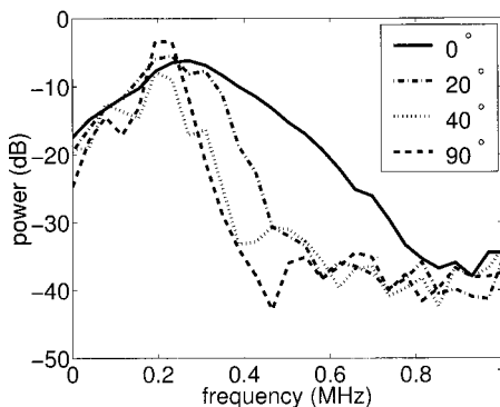
FIG. 3. Power spectra of the 5 cm offset data for four propagation angles relative to the grooves.
