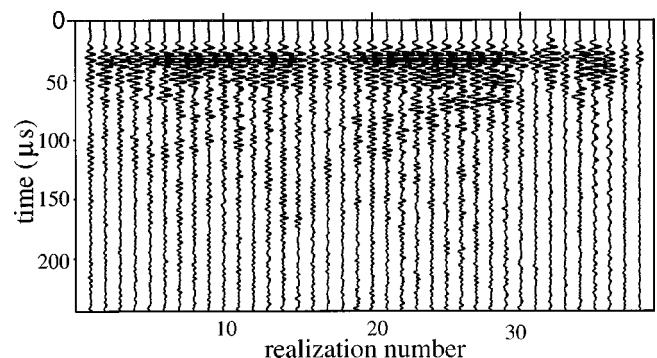
FIG. 5. 38 traces recorded at a fixed offset of 5 cm on the block. The source/receiver combination was offset by 2 mm between shots.
