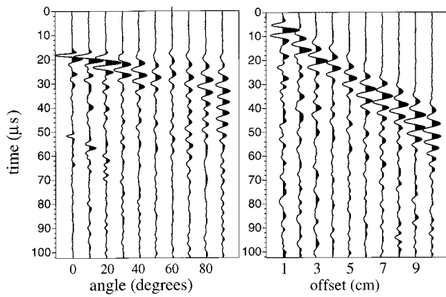
FIG. 2. On the right is a constant-angle section (50°); that is, variable source–receiver distance at a fixed angle relative to the grooves. On the left is a constant-offset section (5 cm offset); that is, variable angles for a fixed source–receiver distance.
