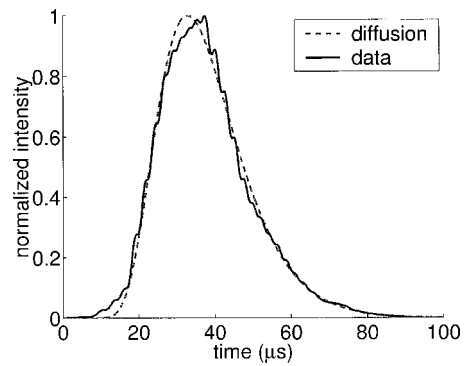
FIG. 7. Fit of intensity to a model involving propagation in a 1D diffusive, attenuative medium. The attenuation is an approximation to diffractive losses off the bottom of the grooves.
