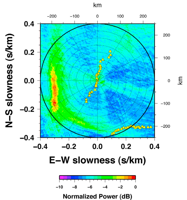
Figure 3. Summation of hourly f-k grids for the same three-day time window used in the crosscorrelations. Yellow triangles show station locations (distance scale on top and right). Dominant energy is from the West, with a secondary source of energy in the Southwest.
